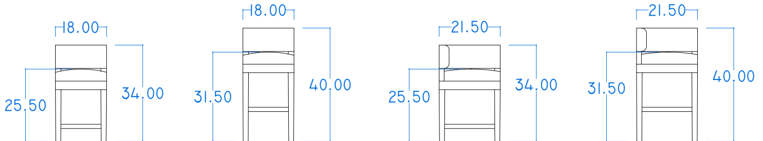
5826-81 ARMLESS BENCH SINGLE RAIL COUNTER HEIGHT
