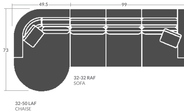
Quarter Inch Scale Drawing
