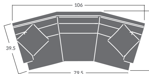
-106 CONVERSATION SOFA W106"
